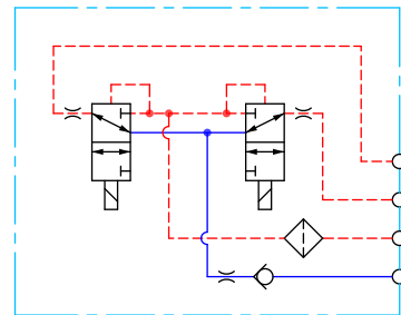
PVEO-R schematic
