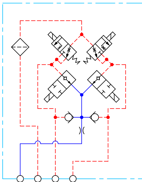
PVEP schematic
